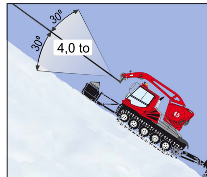
Pulling-force regulator
